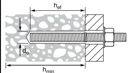
Figure 11 - Installation with (2) washers
