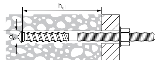
Figure 2 - Hilti HIT-Z and HIT-Z-R specifications
